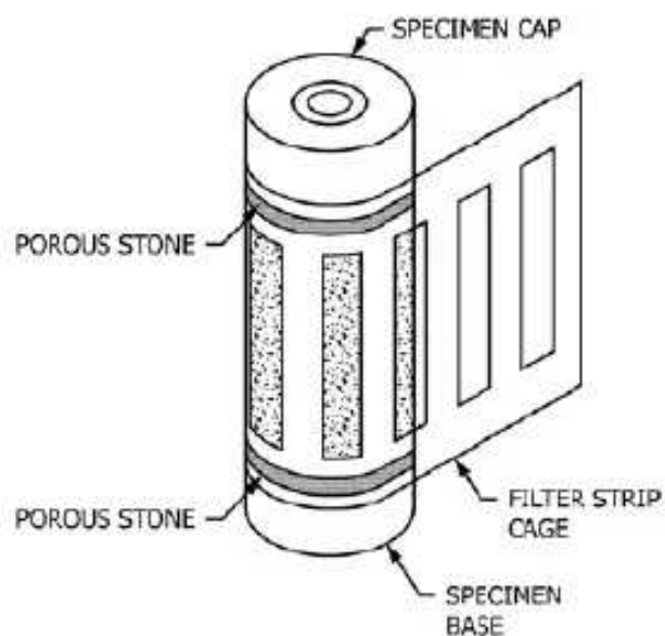
FIG. 2 Filter Strip Cage
