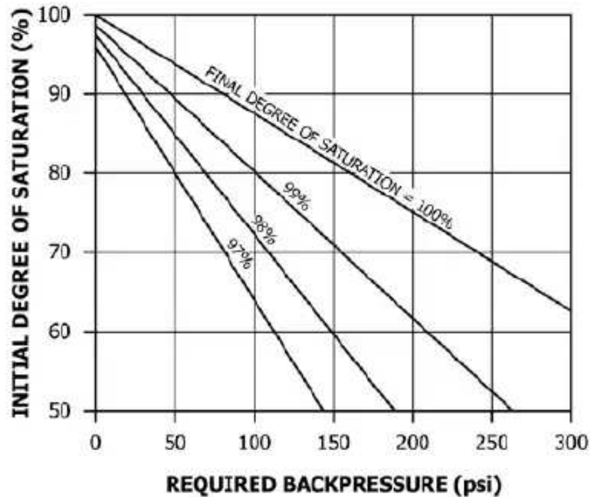
FIG. 3 Pressure to Attain Various Degrees of Saturation
