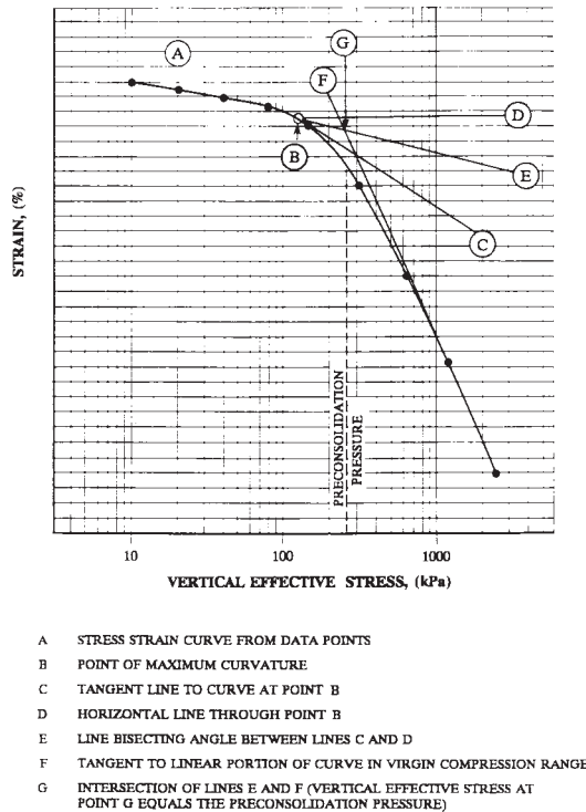
FIG. 4 Evaluation for Preconsolidation Pressure From Casagrande Method
